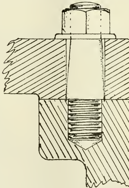
PROPOSED NEW FORM OF STUD
